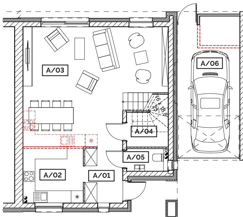
SEGMENT A - PARTER
