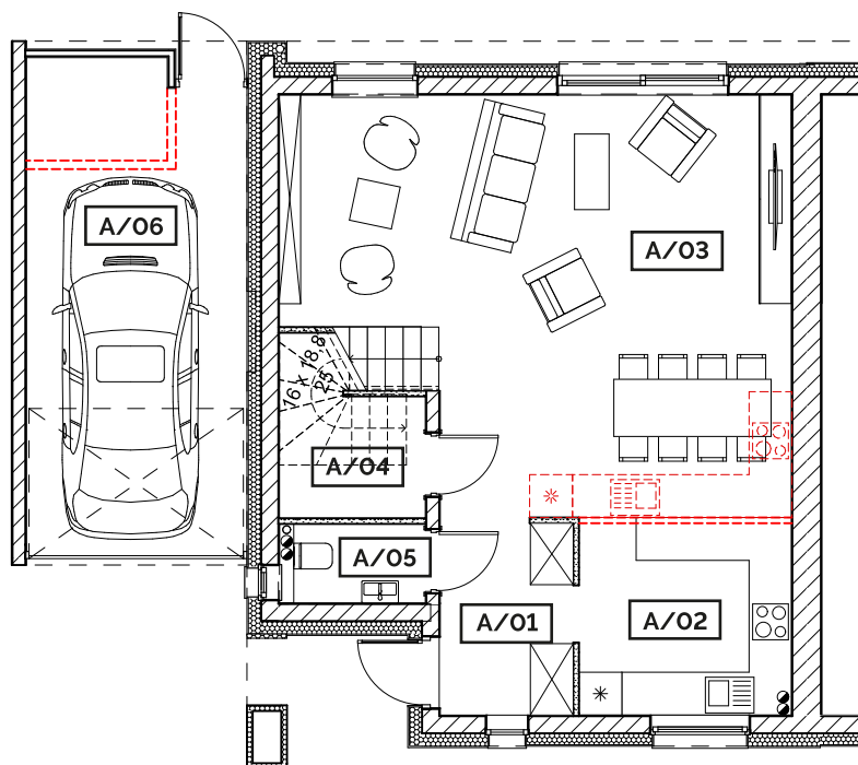
SEGMENT B - PARTER
